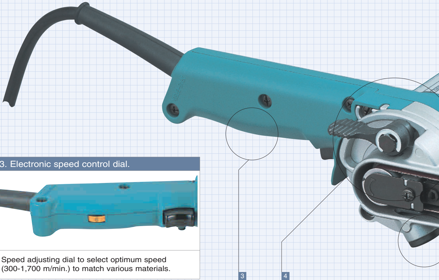
4. Adjustable sanding arm.
