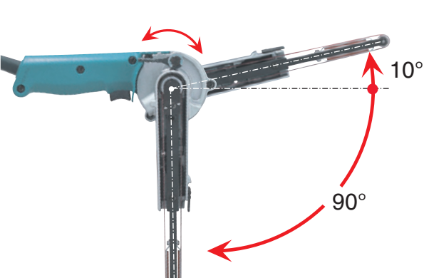
4. Adjustable sanding arm.
